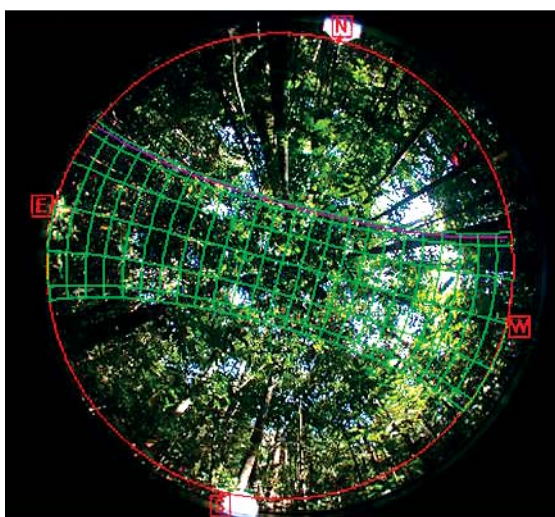
Figure 2b Hemispherical photograph from Sandstone AT-3 (top) and with Granite AT-9 (bottom) with solar trajectory imposed (Annual = Green, Daily for July 8 = Pink).
